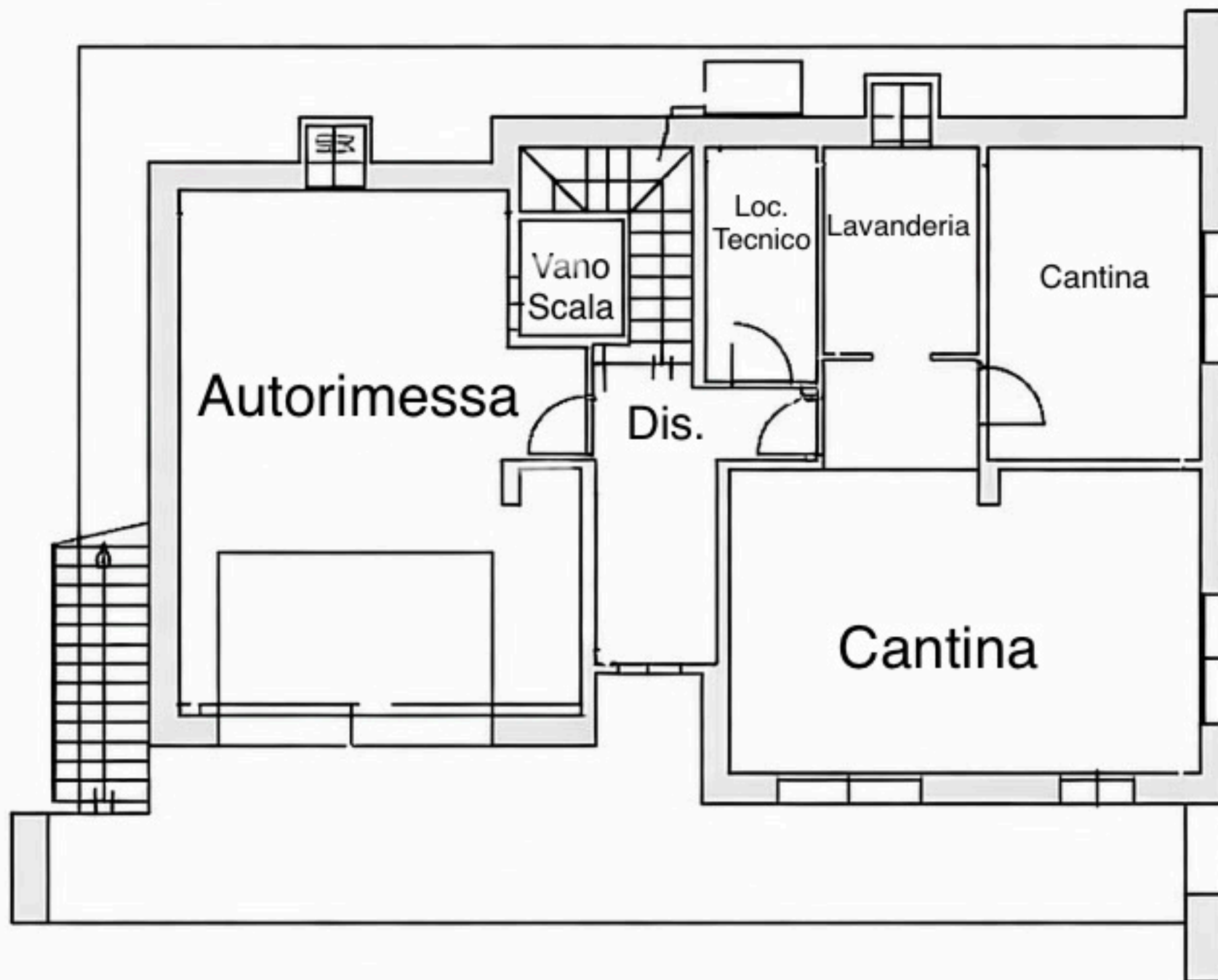
PIANO SEMINTERRATO
